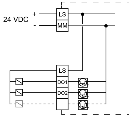
24 V= power supply and 24 V= relay
