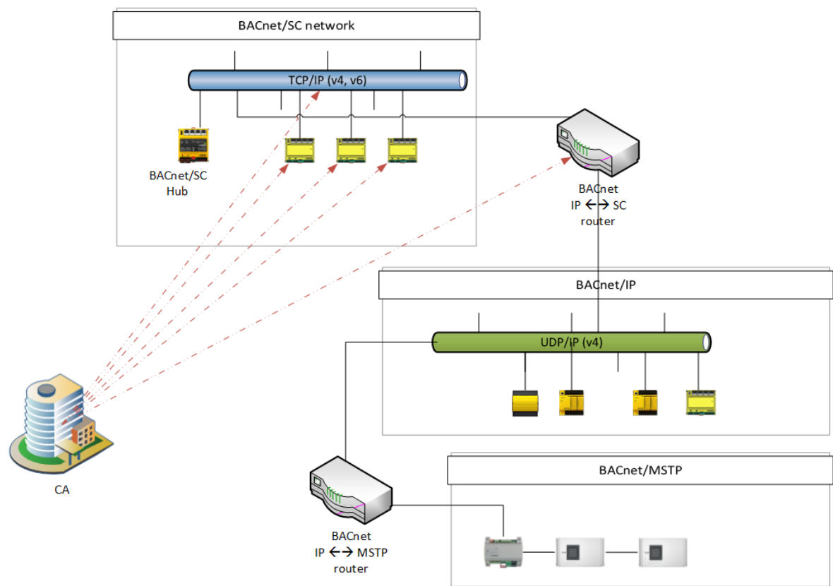
Figure 3 Various BACnet networks and devices
