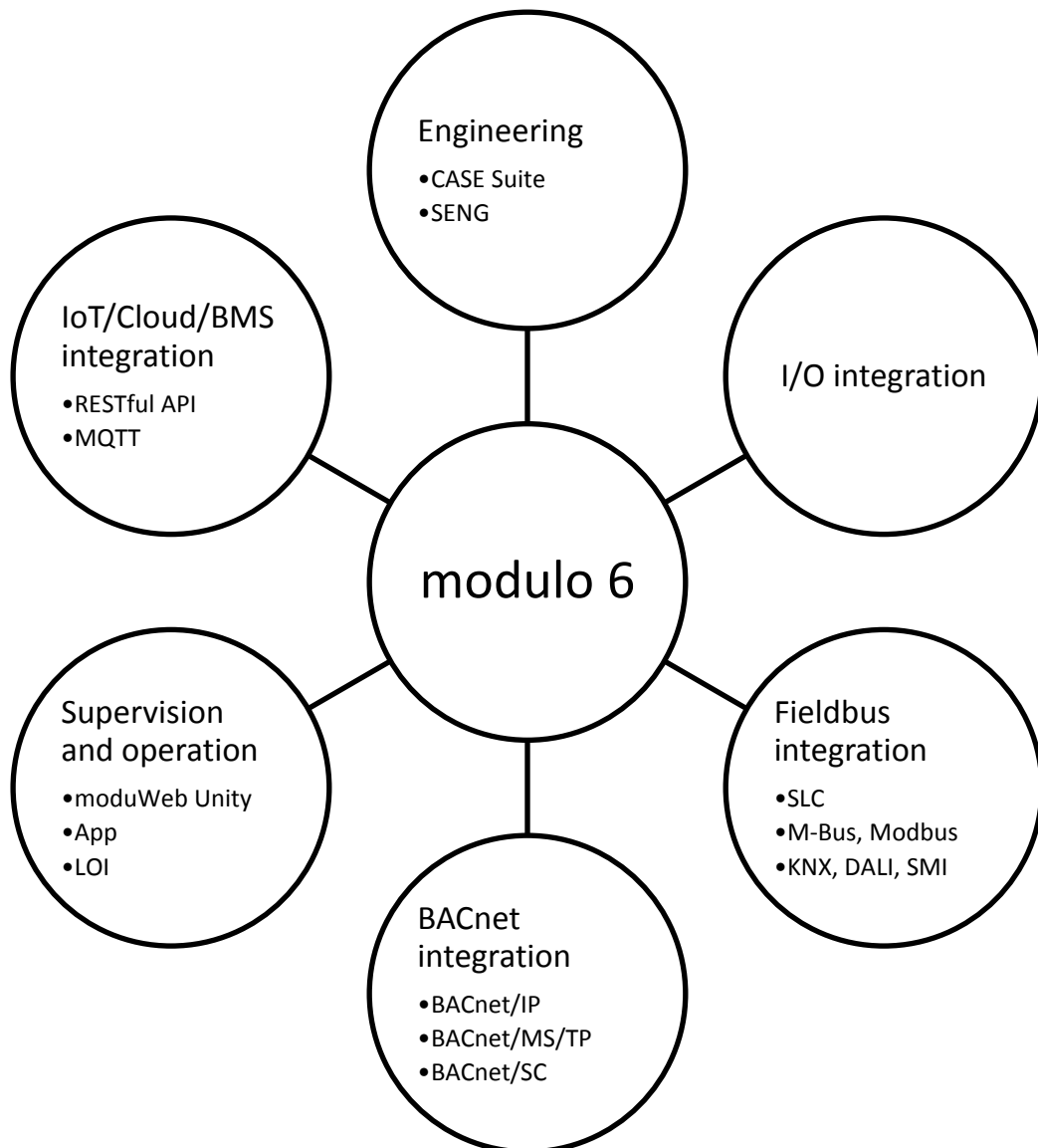
Figure 1 modulo 6 connectivity.
