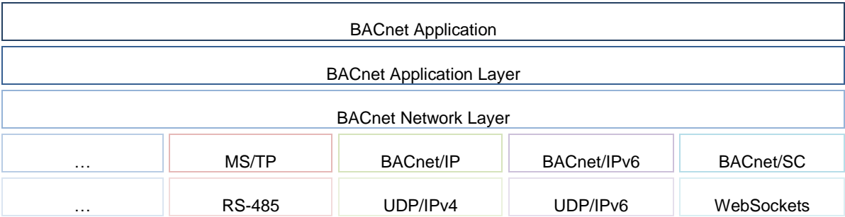
Figure 5 Representation of the different BACnet layers in the OSI layer model
